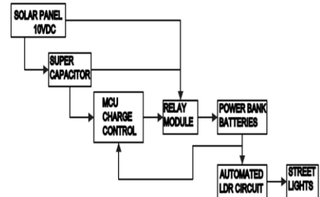
Figure 2: Relay control set-up.
