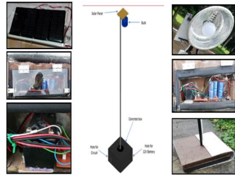
Figure 4: Prototype construction Set-up.
