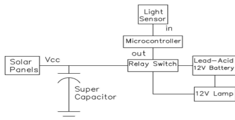
Note: Proposed Two (2) Initial Hardware Designs. Figure 1: Microcontroller set-up.
